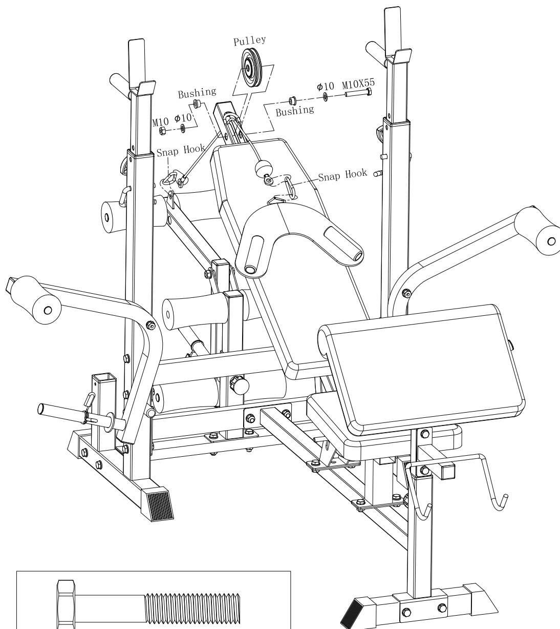
Hex Bolt (M10*55) - 1PCS
